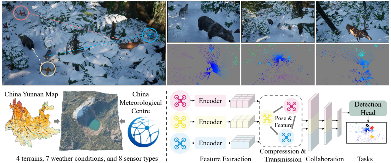
Figure 1: U2UData is collected by performing swarm UAVs autonomous flight tasks in the U2USim environment. Top left: Swarm UAVs autonomous flight task, where each UAV protects an animal based on the arrow. Top right: First-person views and LiDAR images of each UAV. Bottom left: U2USim, a real-world mapping swarm UAVs simulation environment. Bottom right: Swarm UAVs cooperative perception benchmark.
